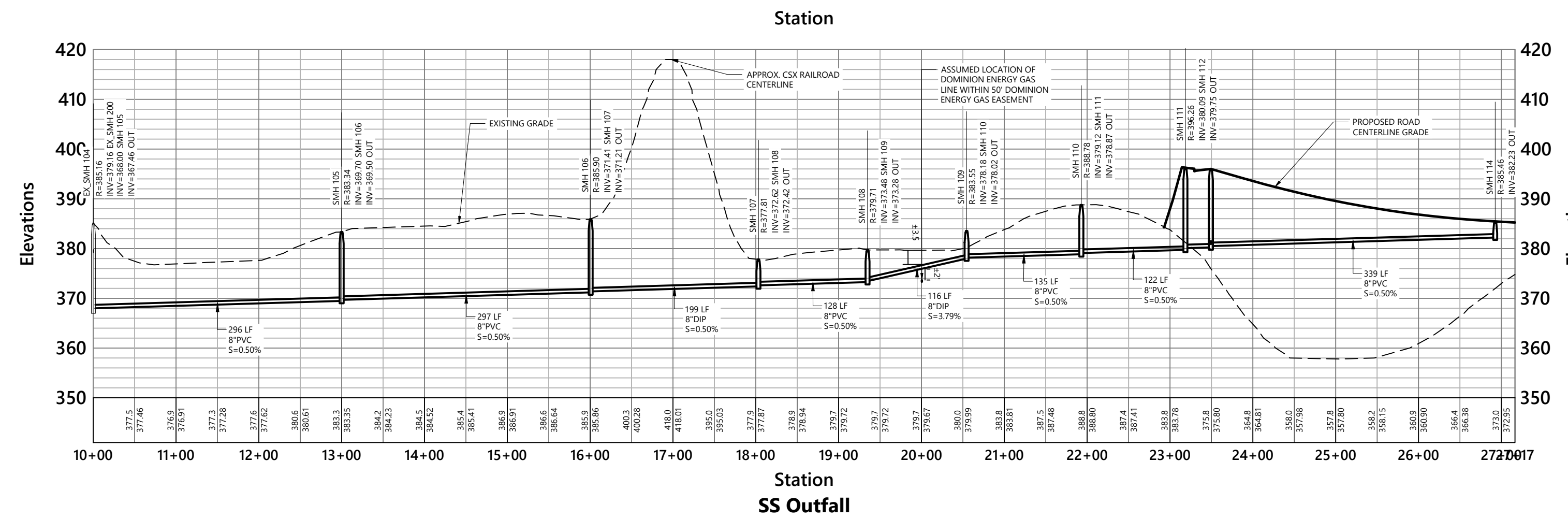
Sewer Outfall Profile
