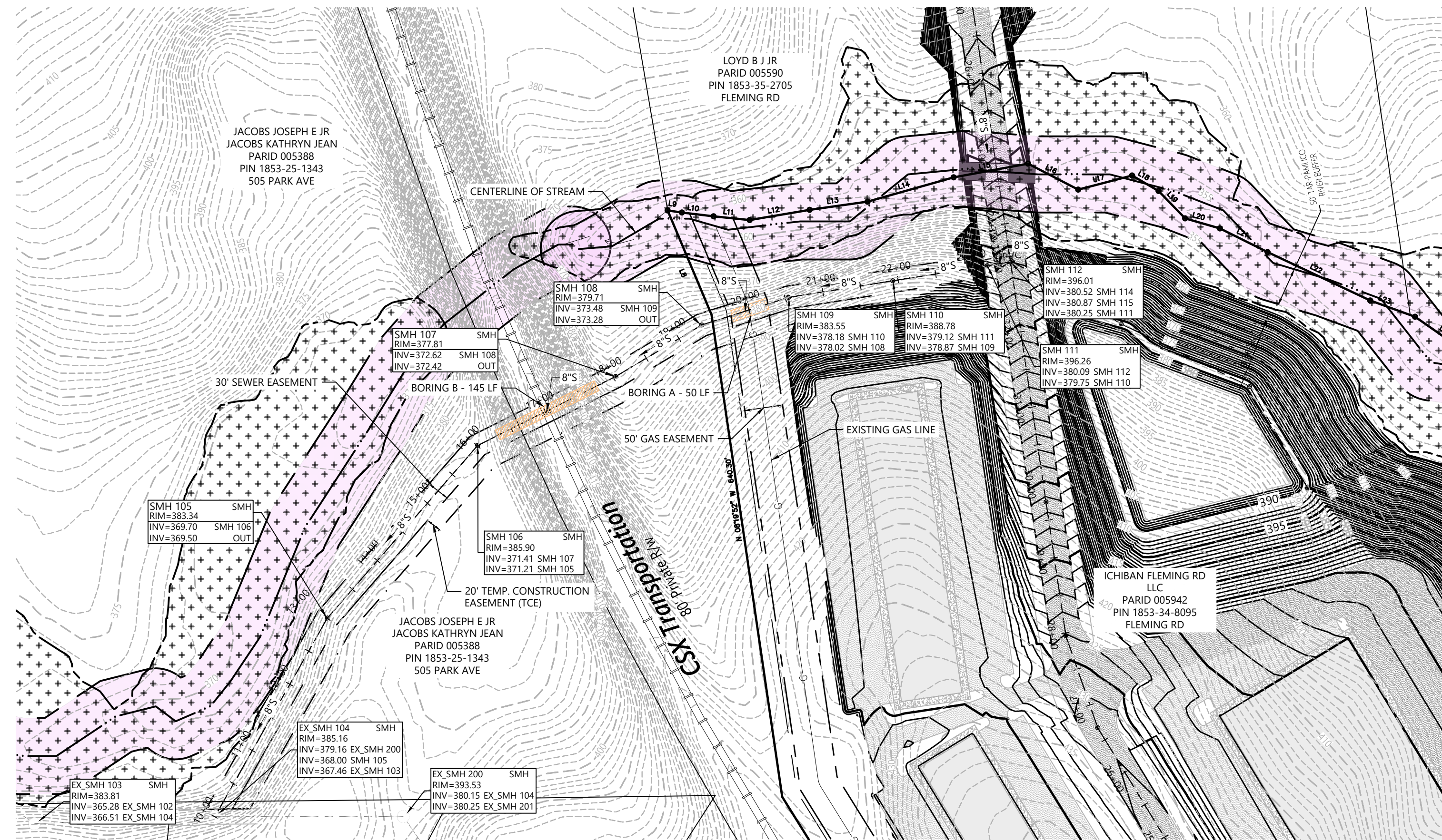
Sewer Outfall Plan
